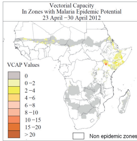
Figure 5. Vectorial capacity map VCAP provided for the epidemic zones of Africa at 1 km spatial resolution.
