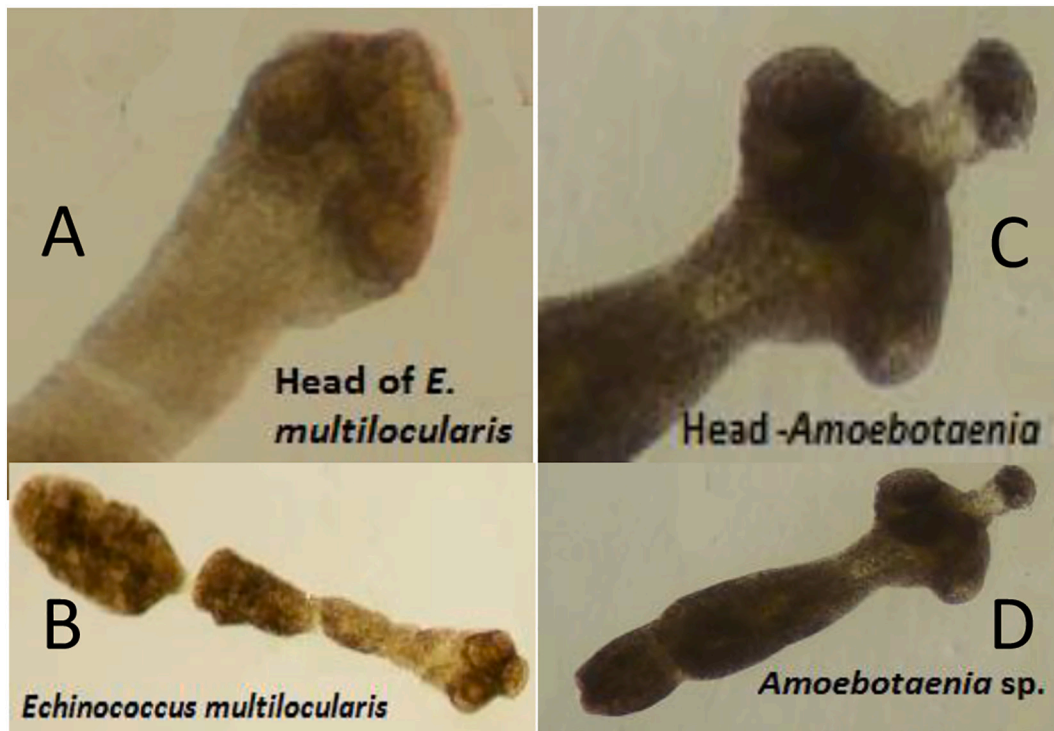
Fig. 1. Morphological differentiation between Echinococcus multilocularis (A,B) and Amoebotaenia sp. (C,D) based on worm size, the shape of and the number of hooks on the scolex and the number and shape of the proglottids (source: French National Reference Laboratory (NRL) for Echinococcus spp.)
