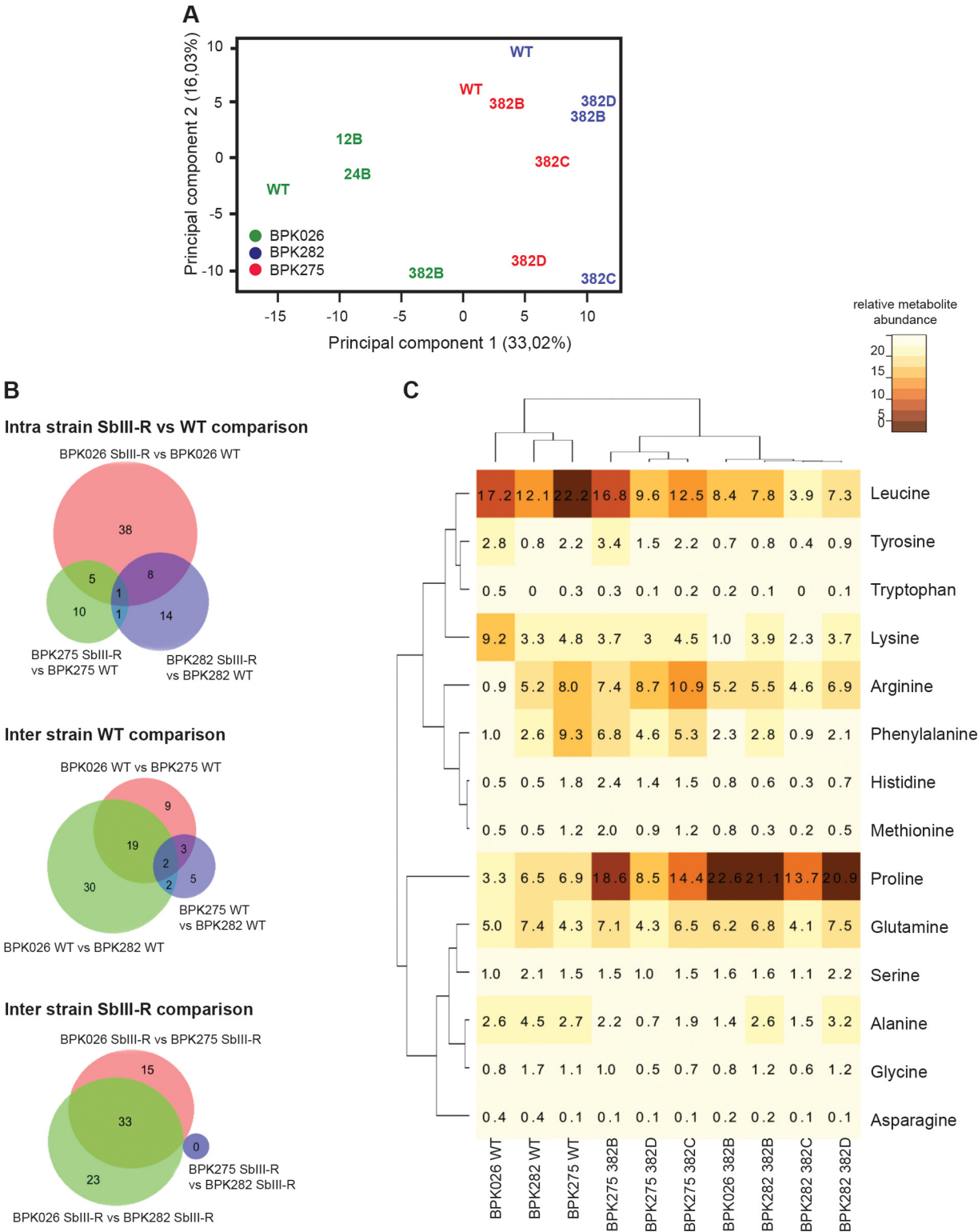
FIG 5 Metabolomics analysis of the selected Sb III -resistant strains. (A) Principal-component analysis based on 300 metabolites and including the initial parental strains (WT) BPK026 (green), BPK275 (red), and BPK282 (blue), the final populations resistant to 382 \mu M Sb III (BPK026 382B, BPK275 382B, -C, and -D, and BPK282 382B, -C, and -D) as well as BPK026 intermediates (12B and 24B, respectively, resistant to 12 and 24 \mu M Sb III ). (B) Venn diagrams showing metabolites significantly different between strains. (C) High hierarchical representation of amino acid abundance in the different strains, including the parental strains (BPK026 WT, BPK282 WT, and BPK275 WT) and the selected populations resistant to 382 \mu M Sb III (BPK275 382B, -C, and -D, BPK026 382B, and BPK282 382B, -C, and -D).
